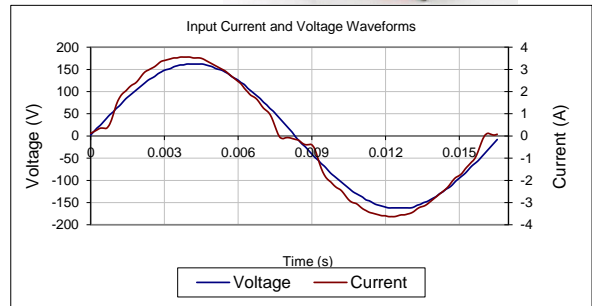
Input AC Current Waveform (ITHD = 9.3%, 50% Load)
